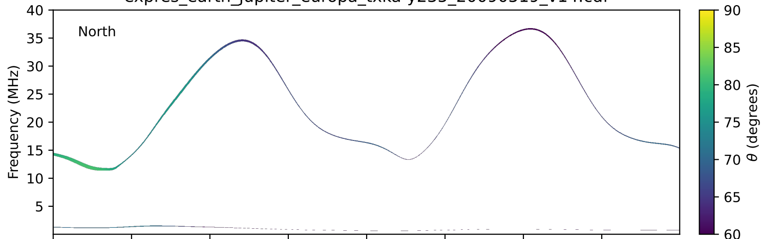
expres_earth_jupiter_europa_txka-y235_20090519_v14.cdf
