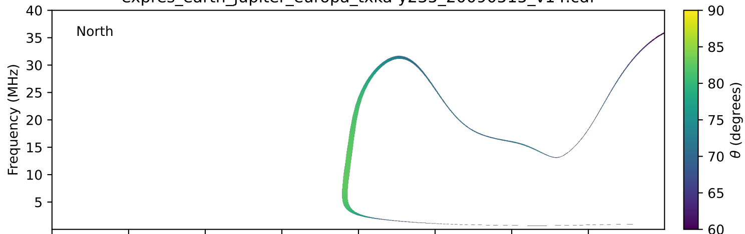
expres_earth_jupiter_europa_txka-y235_20090515_v14.cdf
