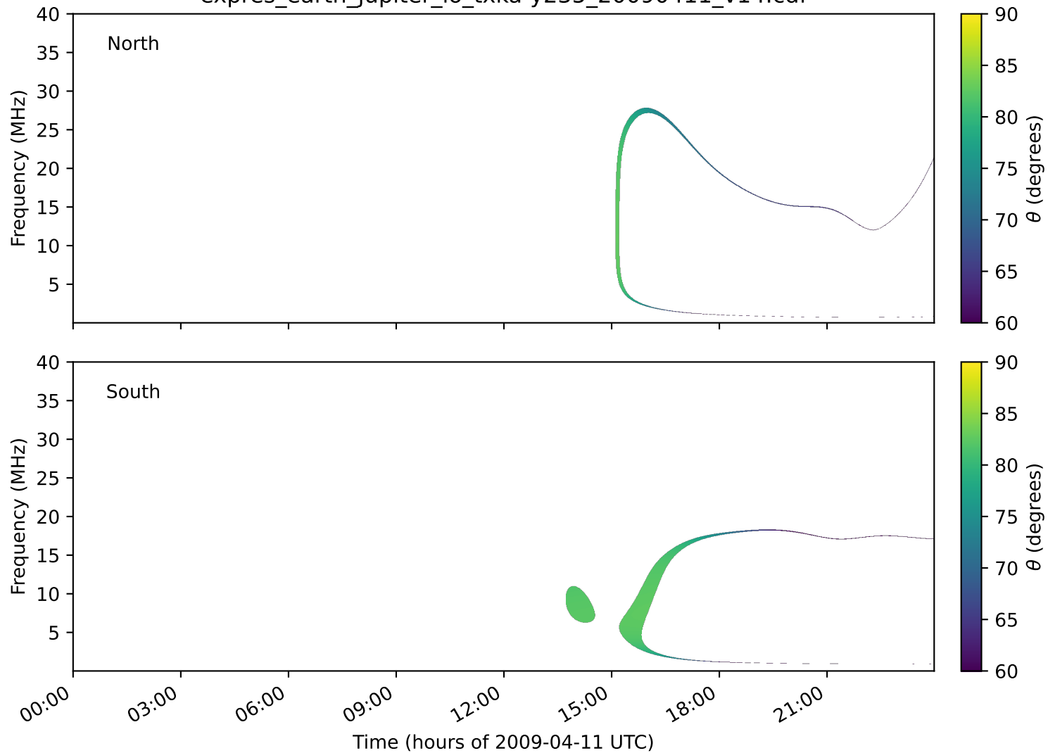
expres_earth_jupiter_io_txka-y235_20090411_v14.cdf
