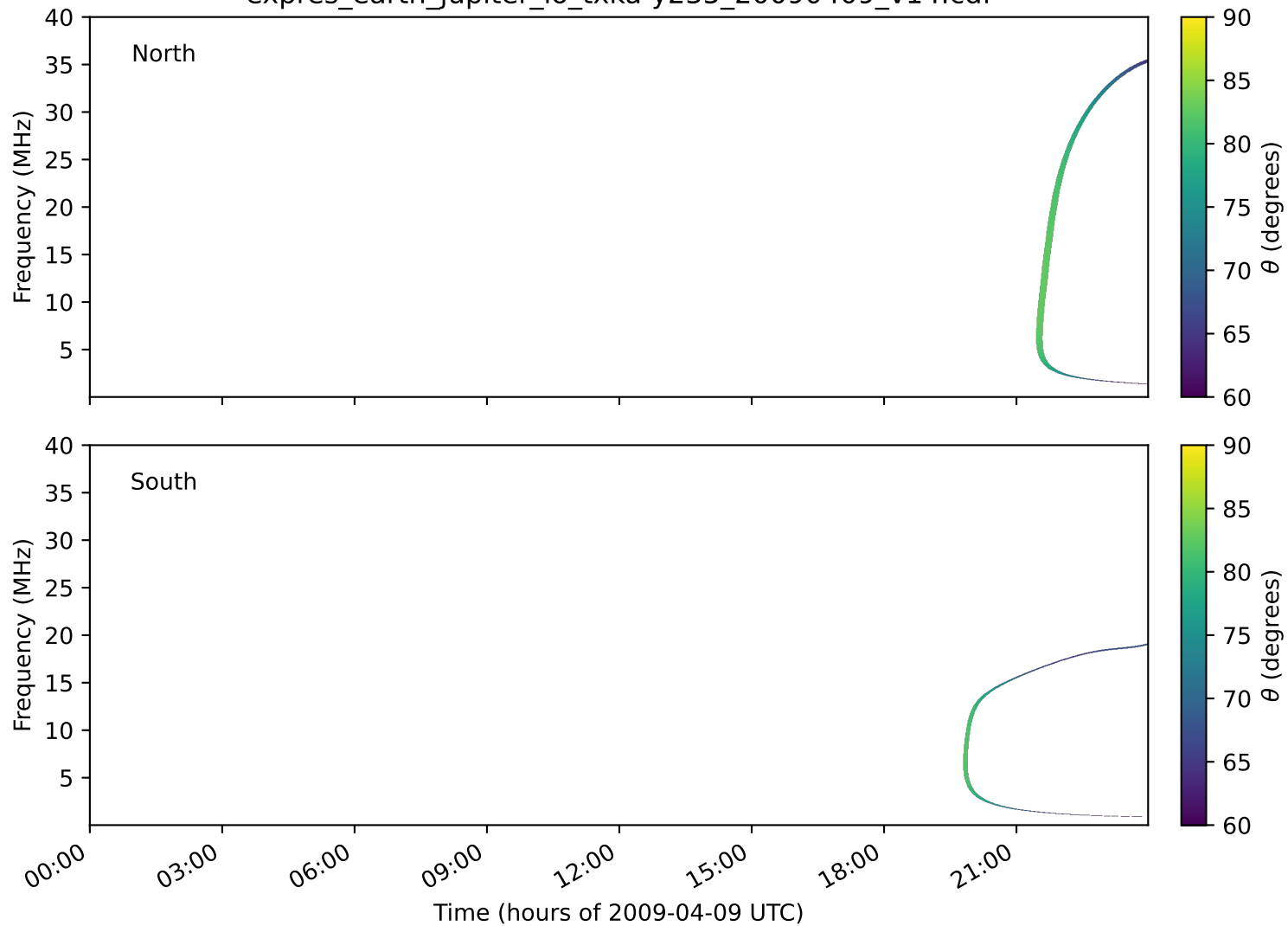
expres_earth_jupiter_io_txka-y235_20090409_v14.cdf
