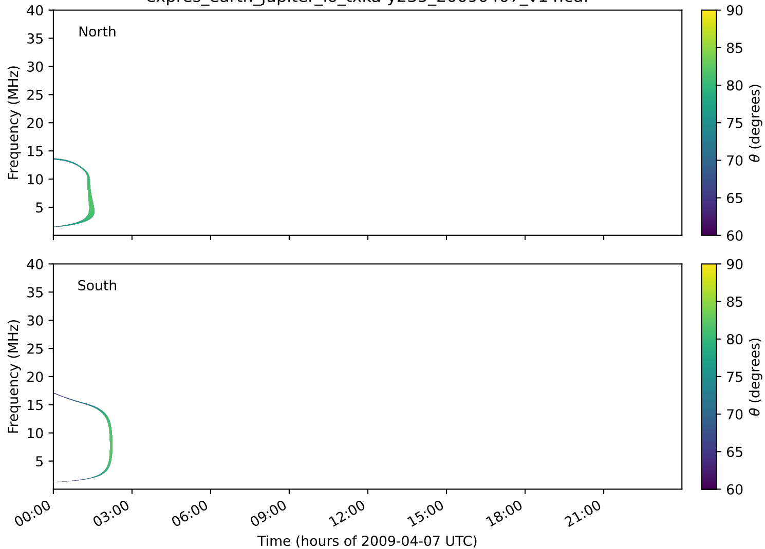
expres_earth_jupiter_io_txka-y235_20090407_v14.cdf
