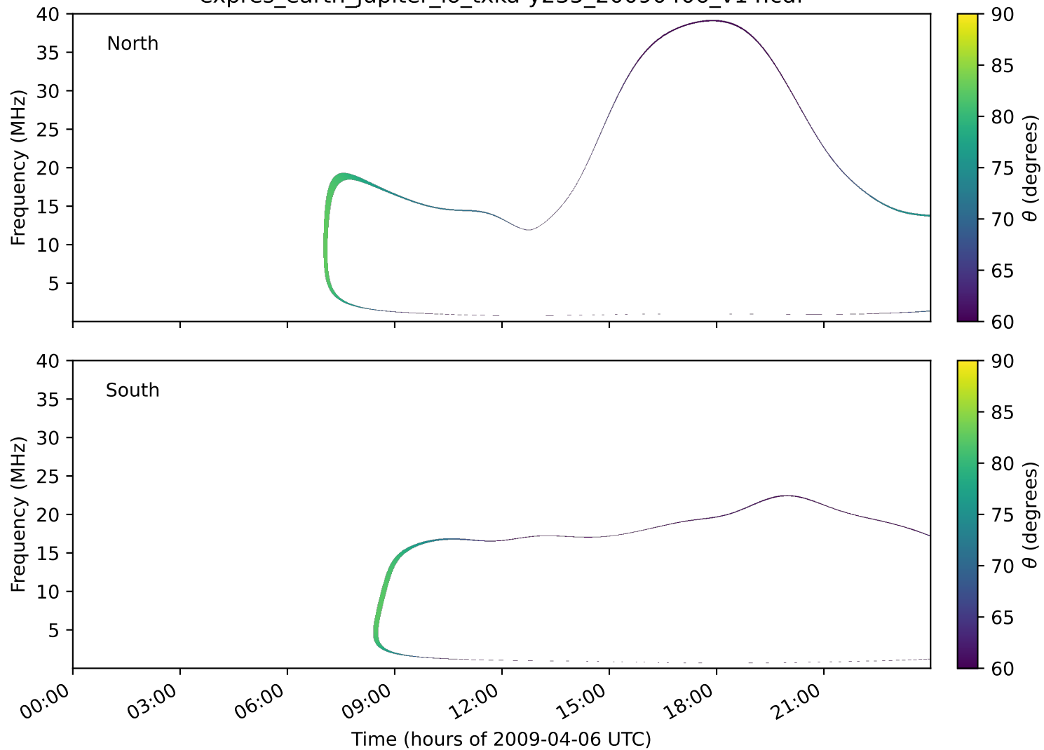
expres_earth_jupiter_io_txka-y235_20090406_v14.cdf
