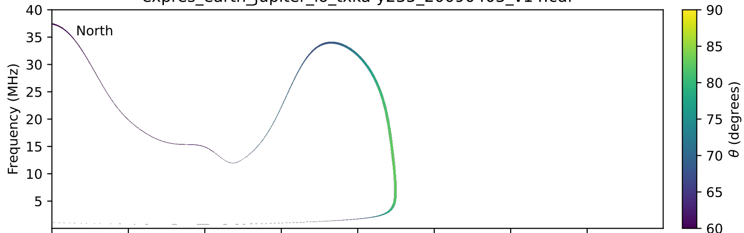
expres_earth_jupiter_io_txka-y235_20090403_v14.cdf
