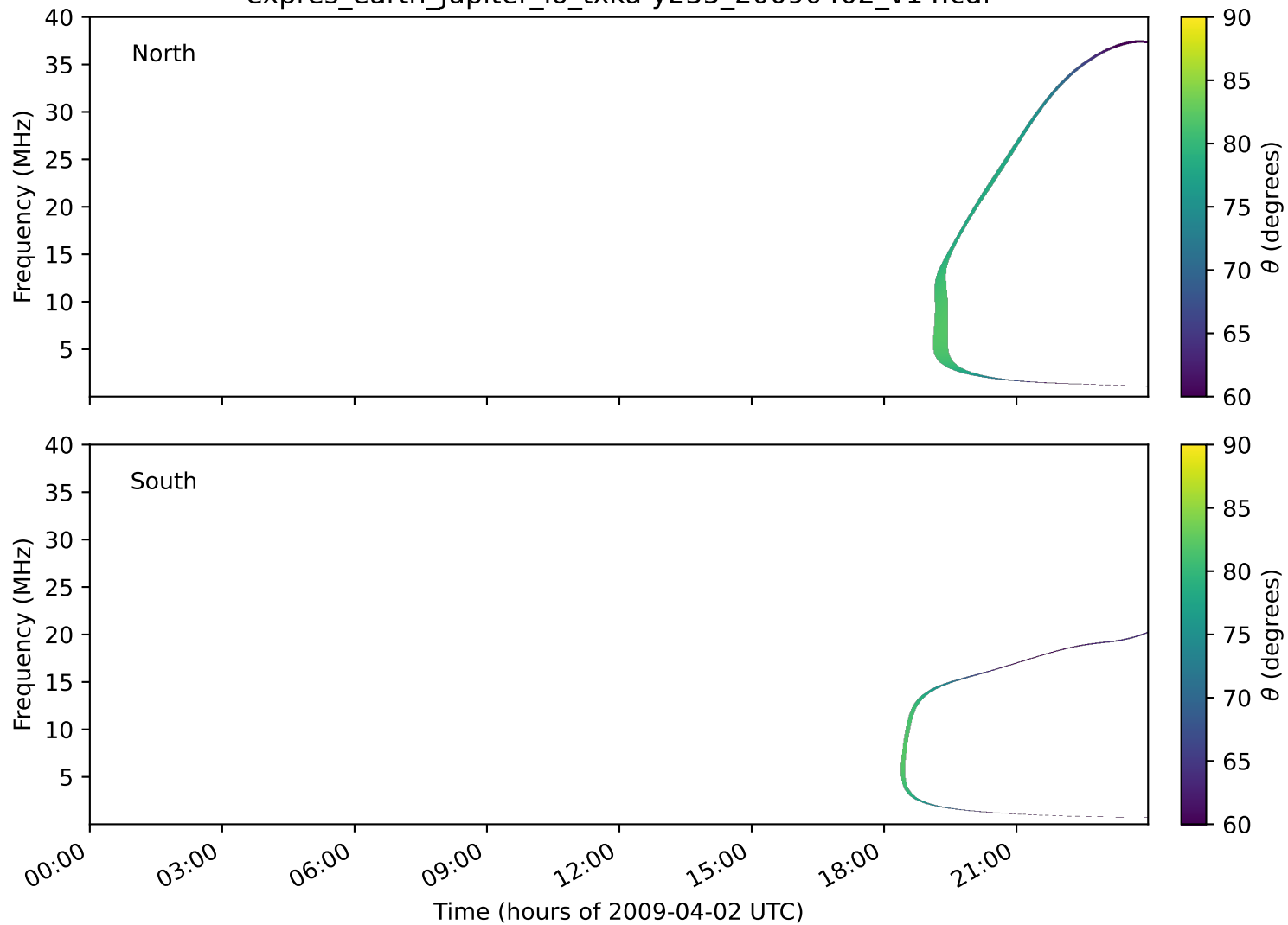
expres_earth_jupiter_io_txka-y235_20090402_v14.cdf
