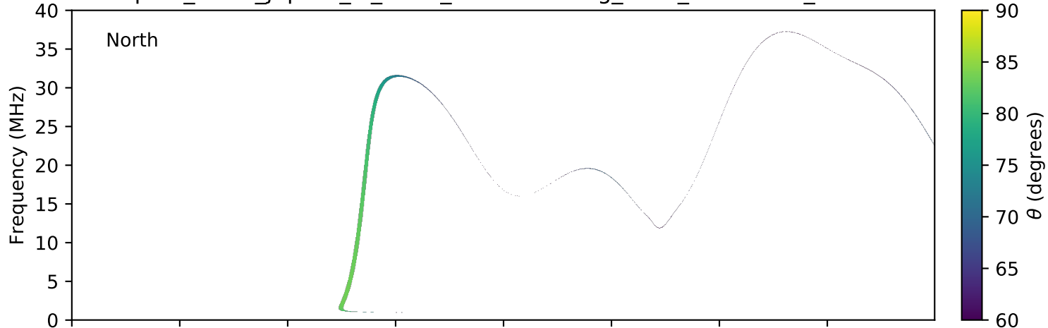
expres_earth_jupiter_io_isaac_lossc-wid1deg_3kev_20090429_v01.cdf
