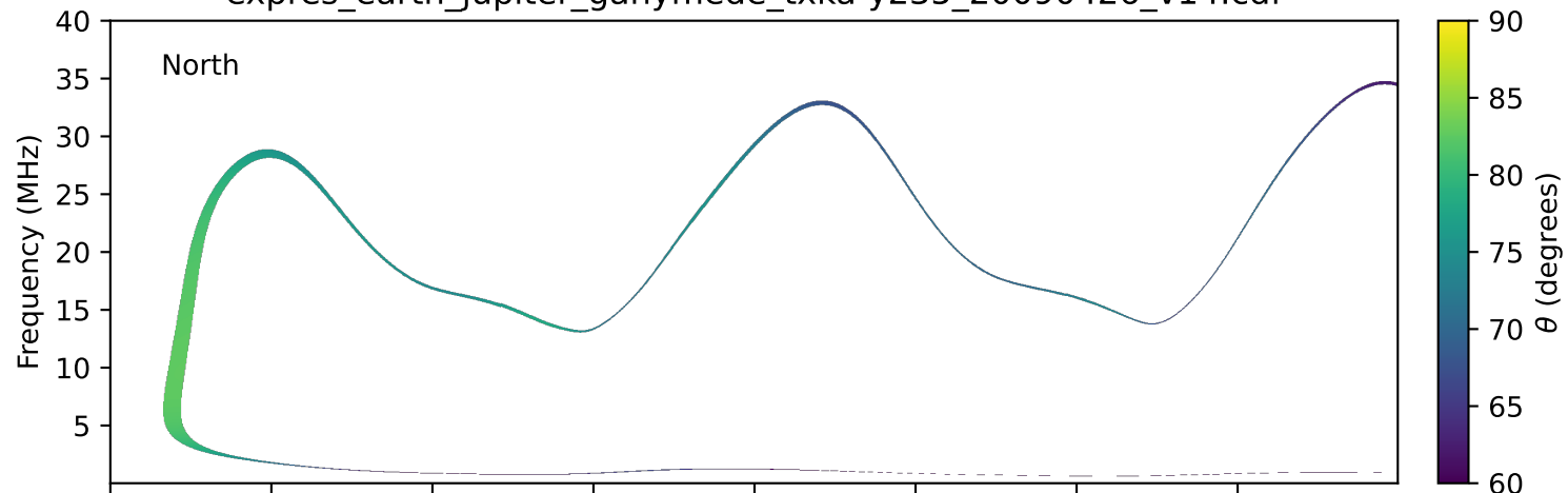
expres_earth_jupiter_ganymede_txka-y235_20090426_v14.cdf
