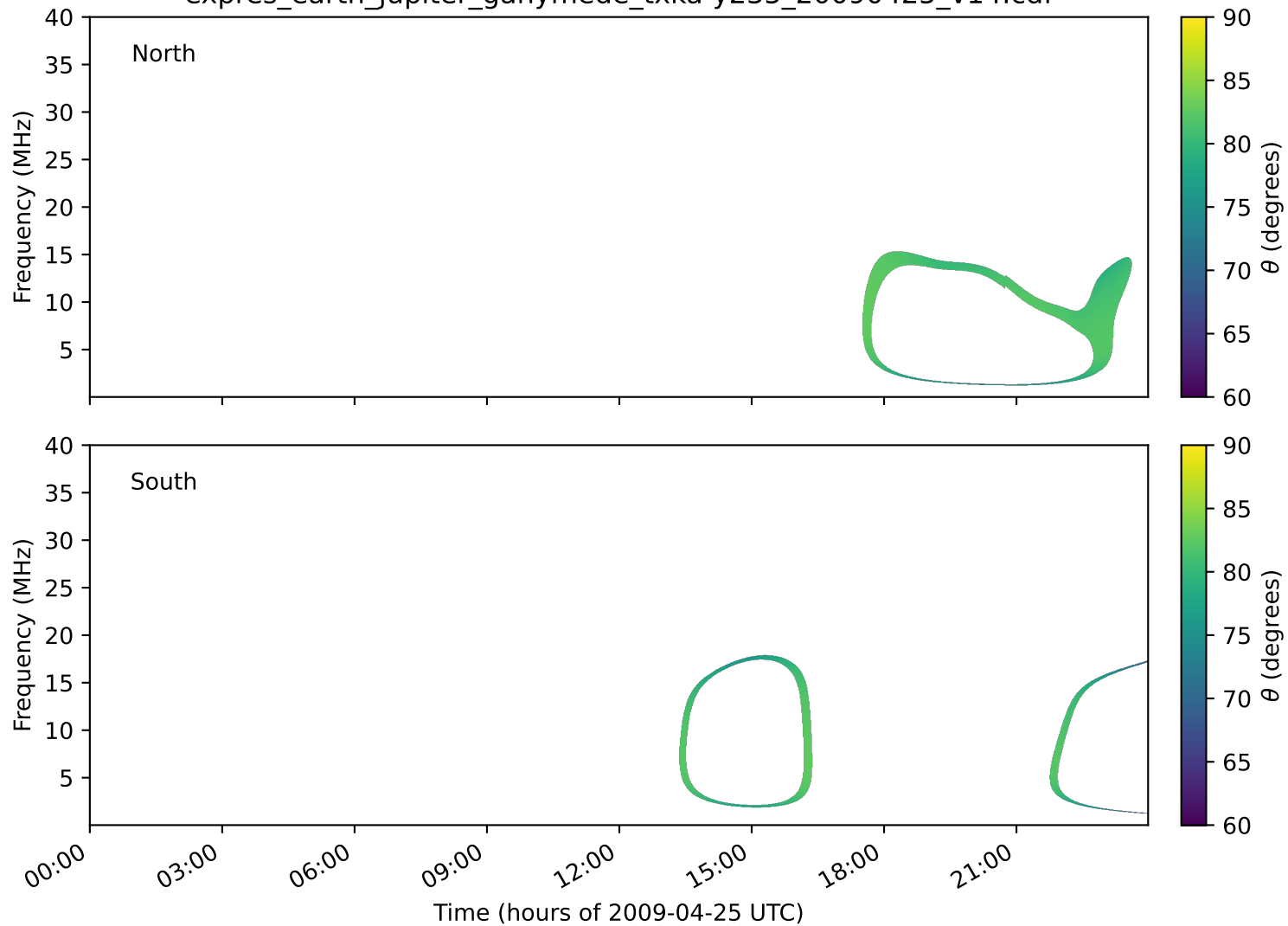
expres_earth_jupiter_ganymede_txka-y235_20090425_v14.cdf
