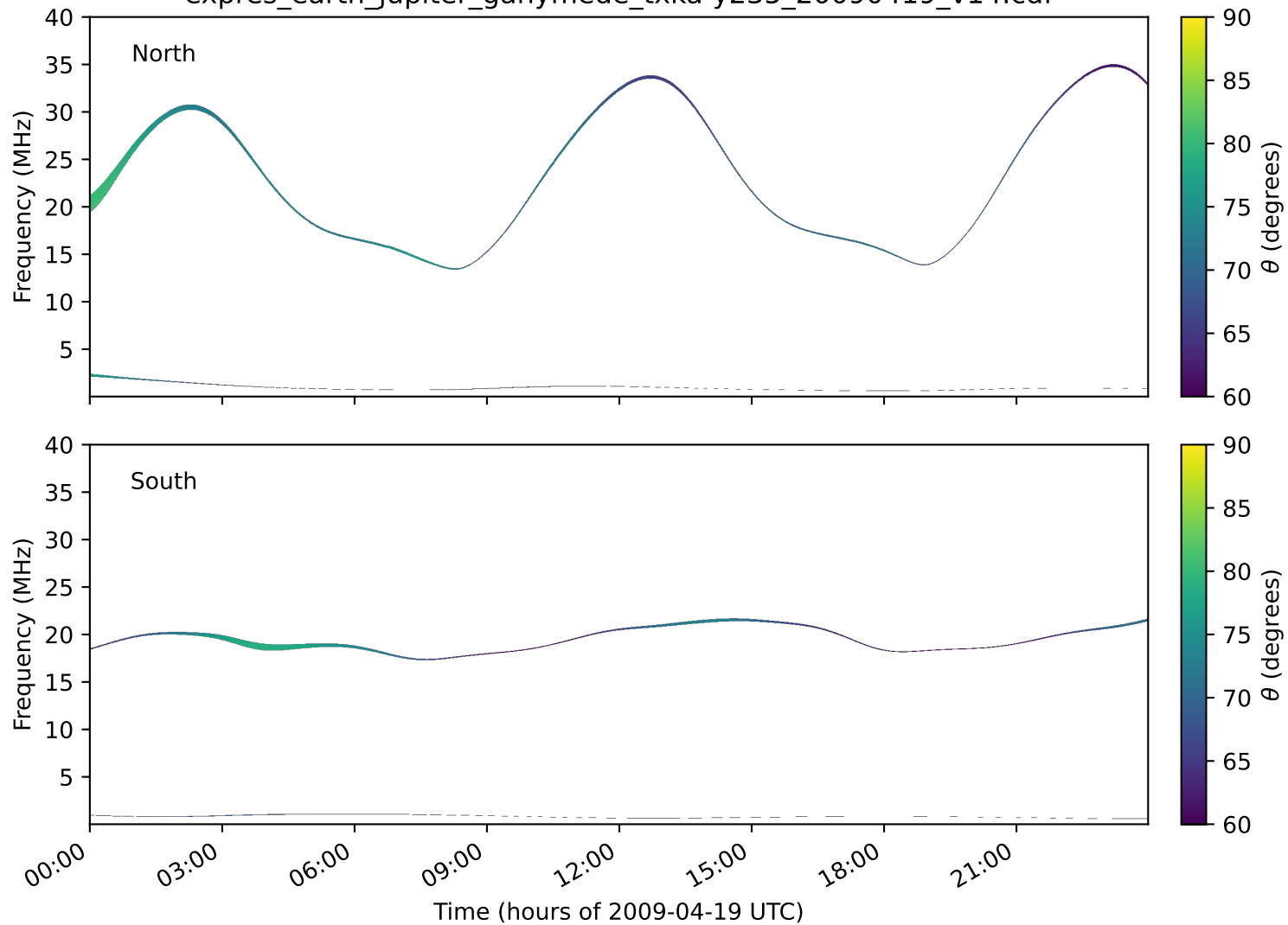
expres_earth_jupiter_ganymede_txka-y235_20090419_v14.cdf
