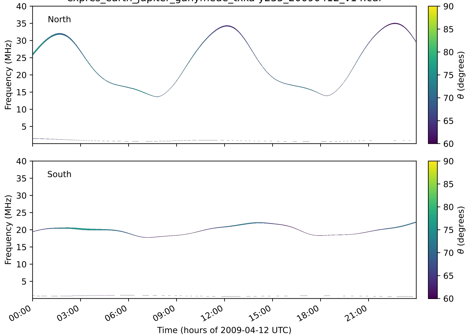
expres_earth_jupiter_ganymede_txka-y235_20090412_v14.cdf
