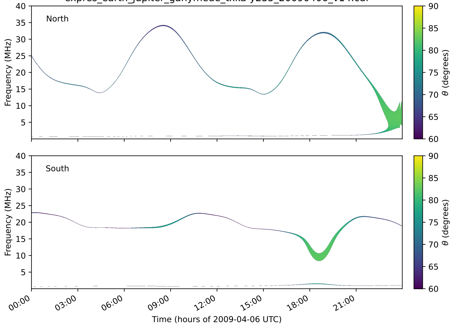
expres_earth_jupiter_ganymede_txka-y235_20090406_v14.cdf
