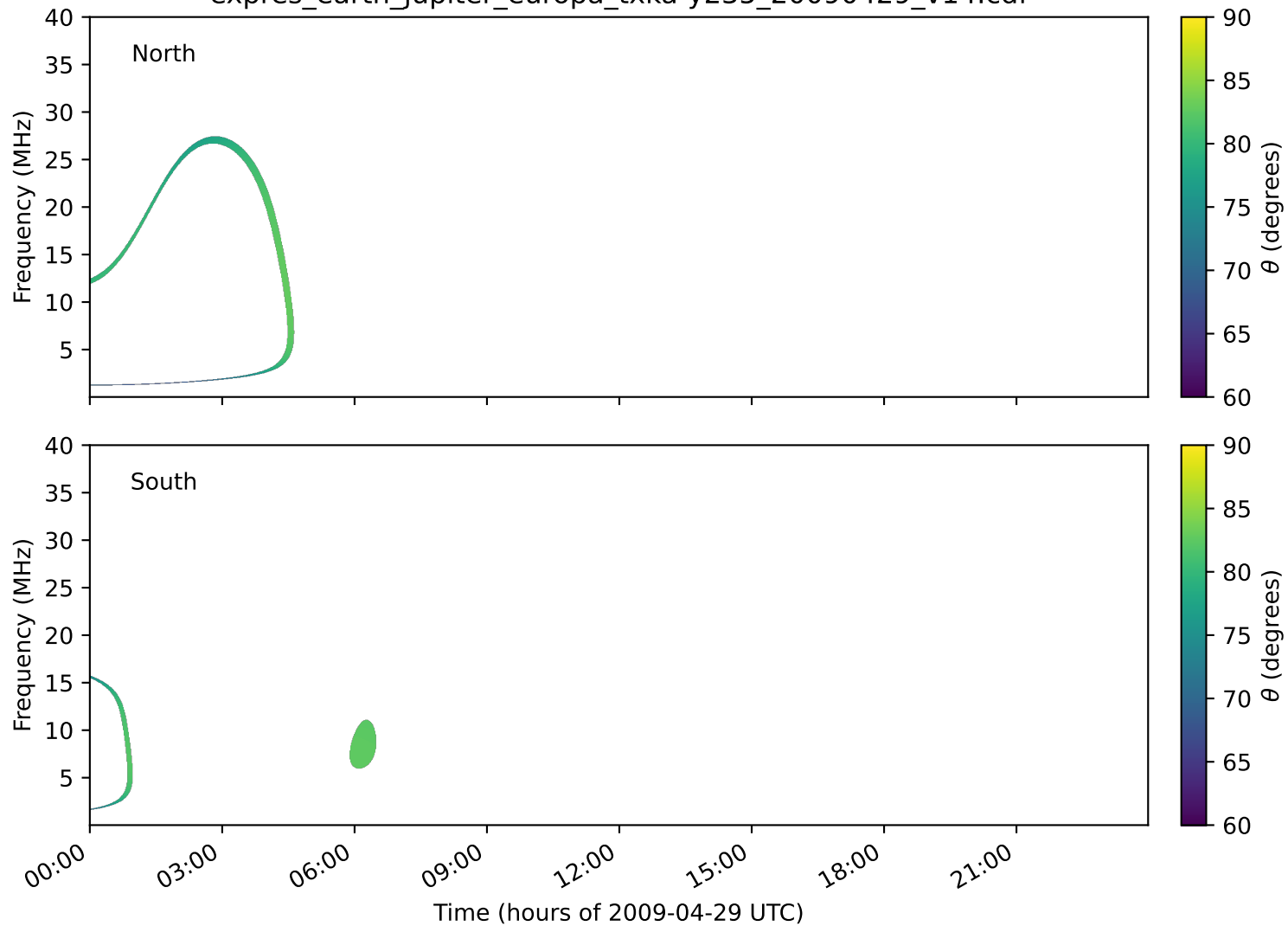
expres_earth_jupiter_europa_txka-y235_20090429_v14.cdf
