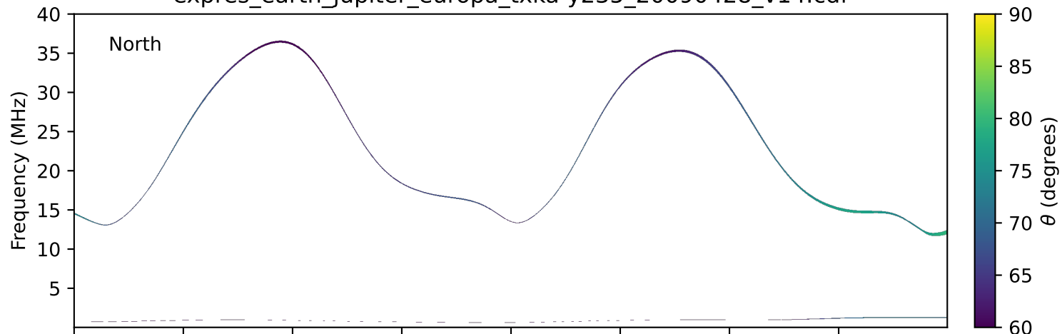
expres_earth_jupiter_europa_txka-y235_20090428_v14.cdf
