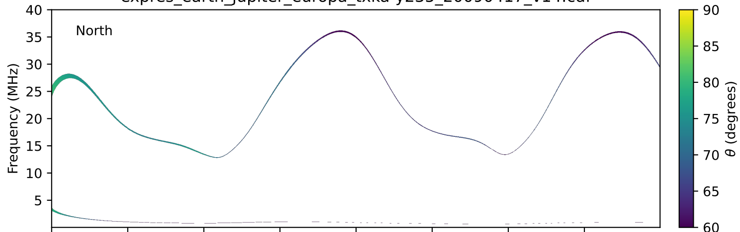
expres_earth_jupiter_europa_txka-y235_20090417_v14.cdf
