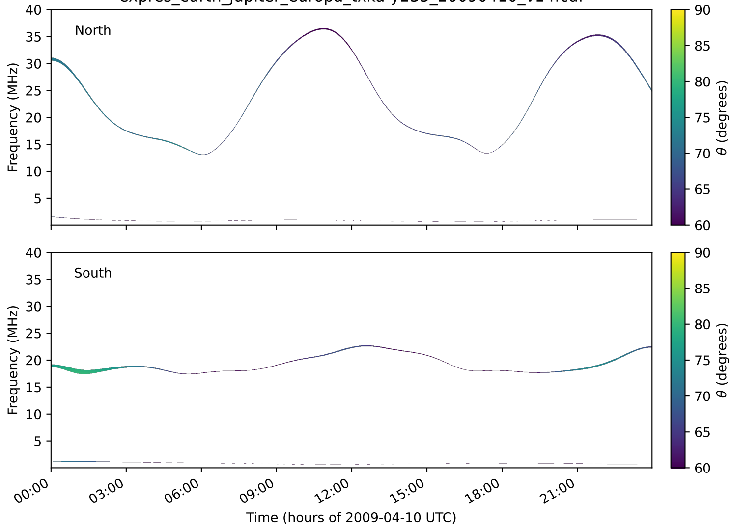
expres_earth_jupiter_europa_txka-y235_20090410_v14.cdf
