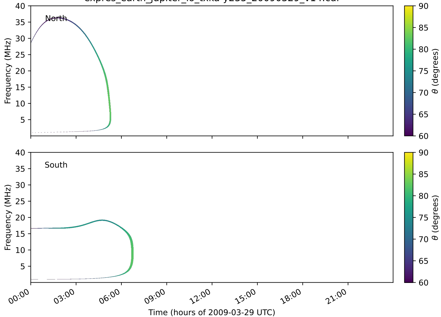
expres_earth_jupiter_io_txka-y235_20090329_v14.cdf
