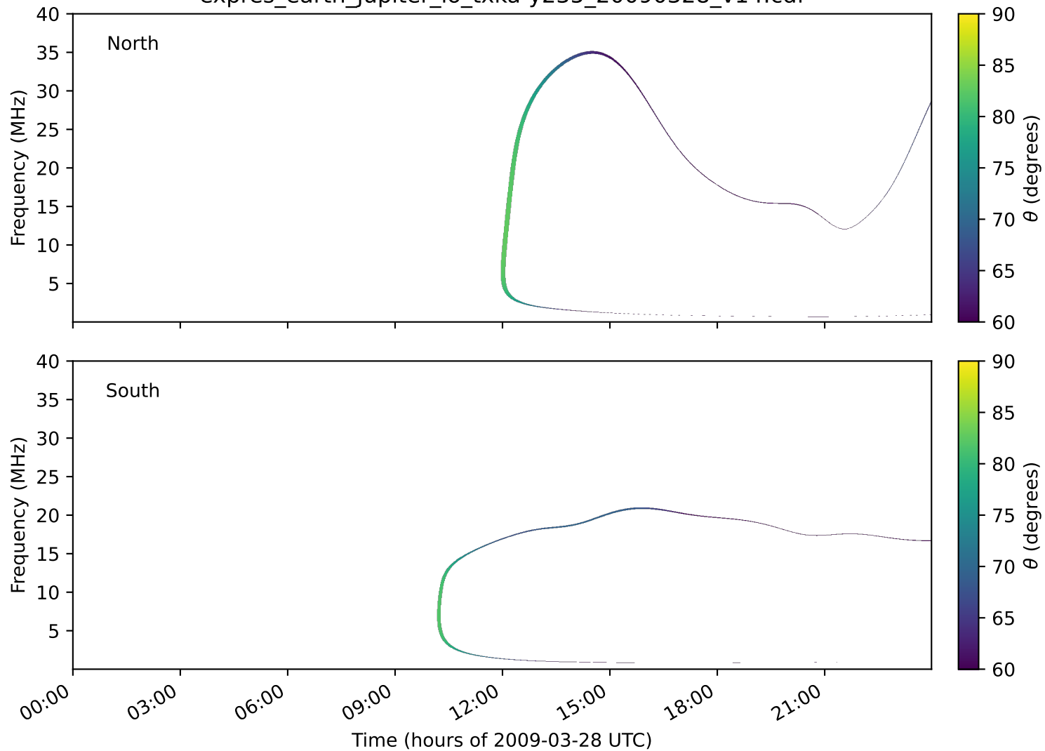
expres_earth_jupiter_io_txka-y235_20090328_v14.cdf
