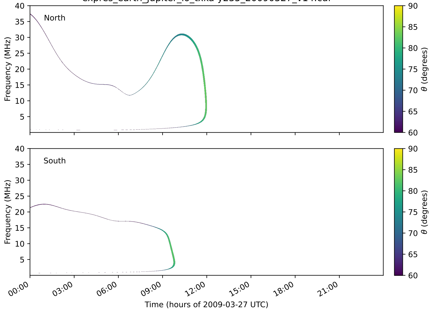
expres_earth_jupiter_io_txka-y235_20090327_v14.cdf
