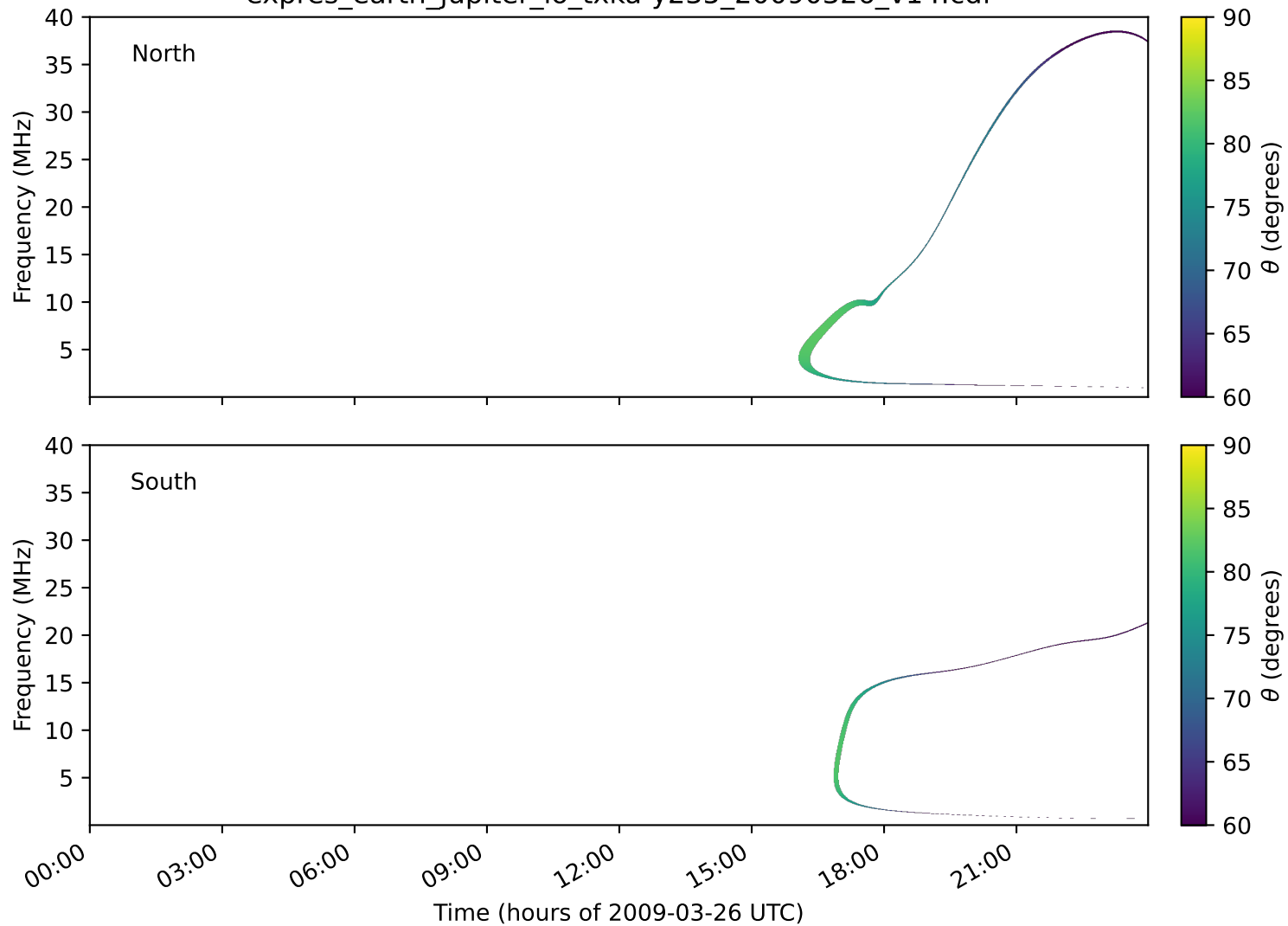
expres_earth_jupiter_io_txka-y235_20090326_v14.cdf
