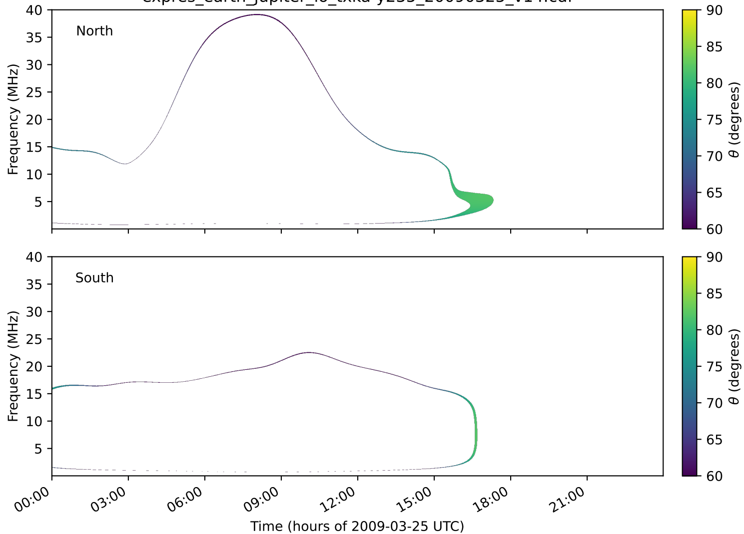
expres_earth_jupiter_io_txka-y235_20090325_v14.cdf
