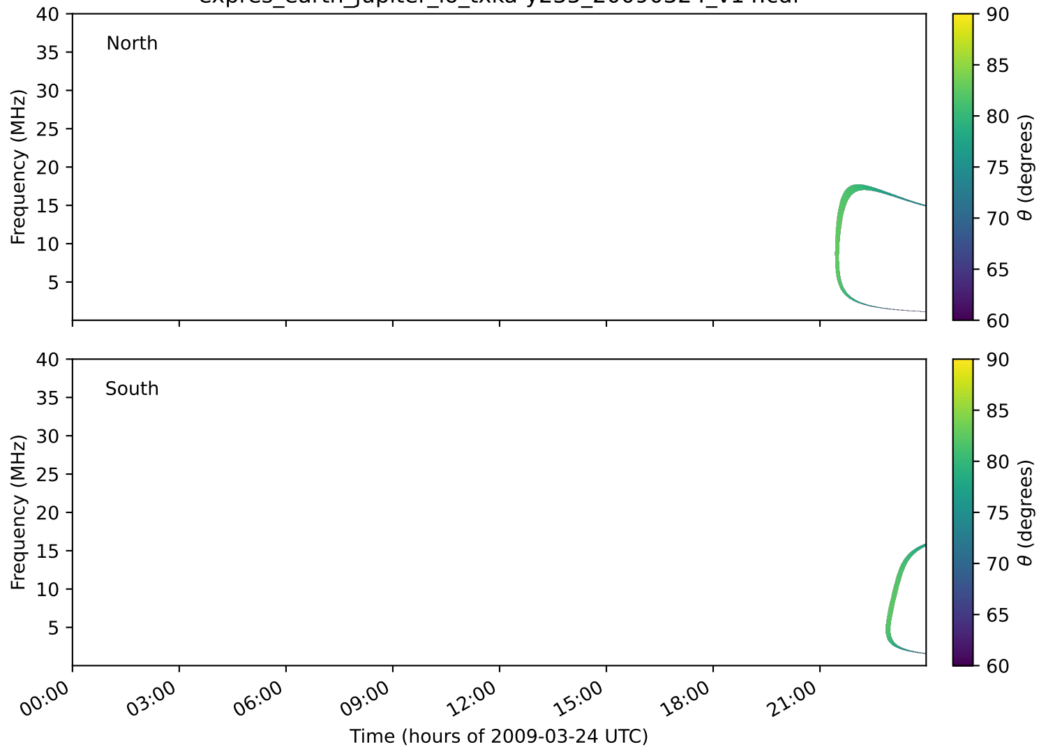
expres_earth_jupiter_io_txka-y235_20090324_v14.cdf
