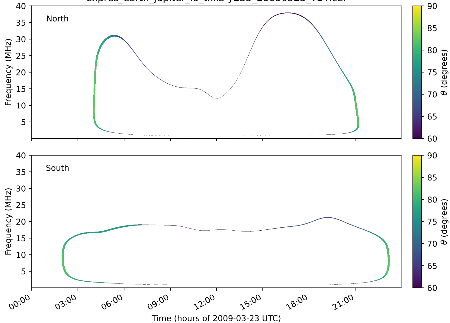
expres_earth_jupiter_io_txka-y235_20090323_v14.cdf
