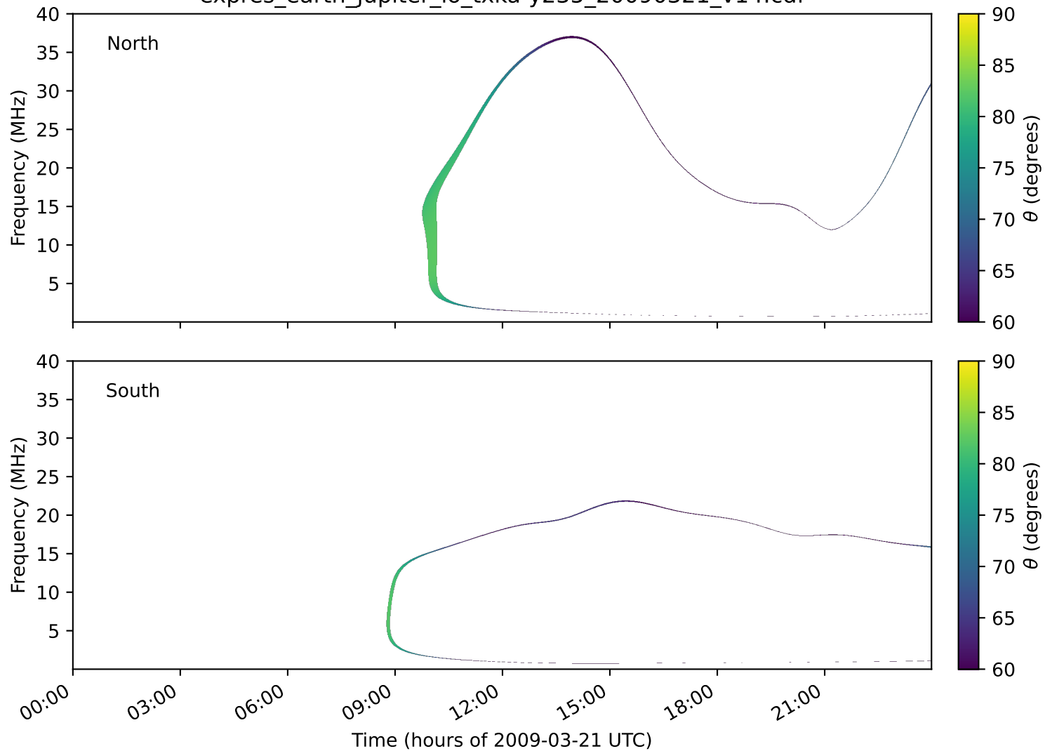
expres_earth_jupiter_io_txka-y235_20090321_v14.cdf
