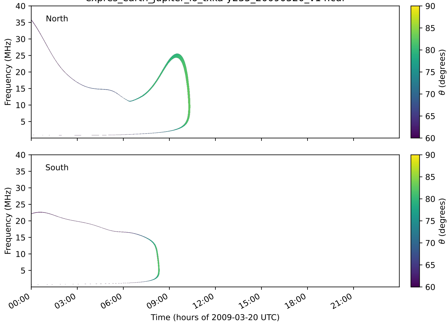
expres_earth_jupiter_io_txka-y235_20090320_v14.cdf
