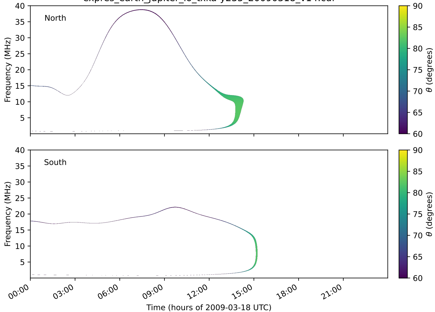
expres_earth_jupiter_io_txka-y235_20090318_v14.cdf
