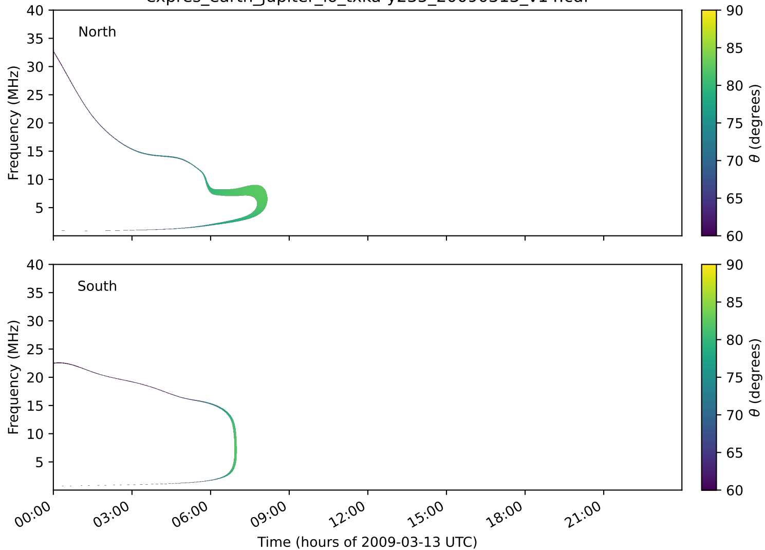
expres_earth_jupiter_io_txka-y235_20090313_v14.cdf
