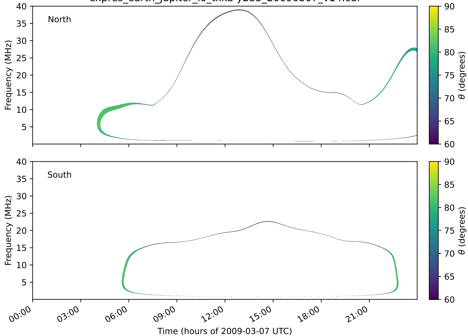
expres_earth_jupiter_io_txka-y235_20090307_v14.cdf
