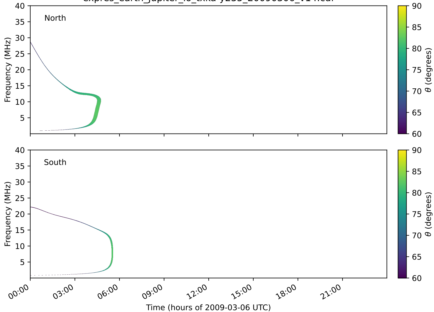
expres_earth_jupiter_io_txka-y235_20090306_v14.cdf
