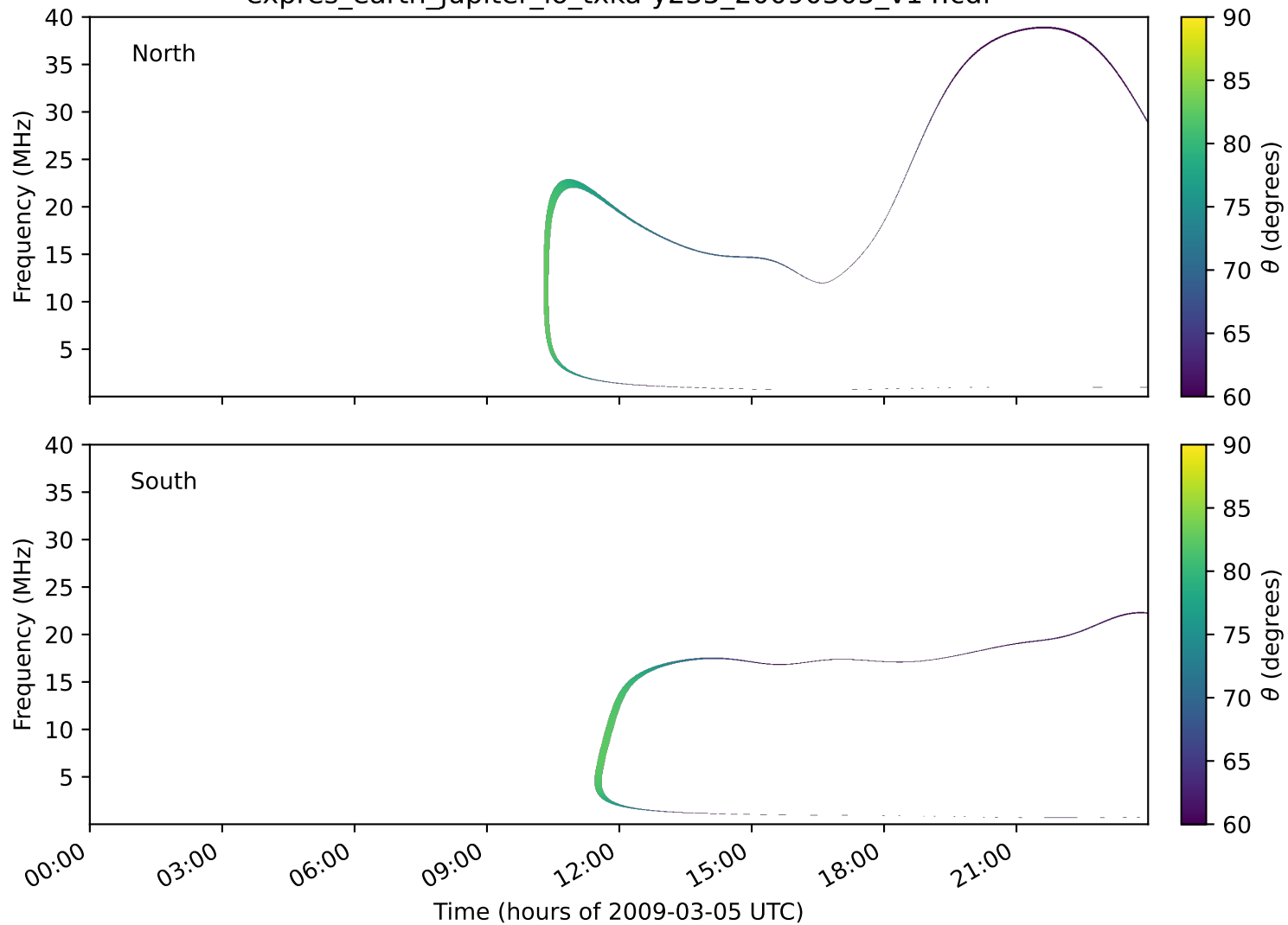
expres_earth_jupiter_io_txka-y235_20090305_v14.cdf
