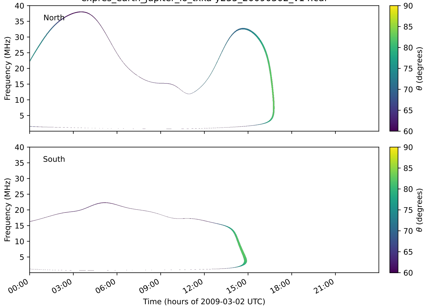
expres_earth_jupiter_io_txka-y235_20090302_v14.cdf
