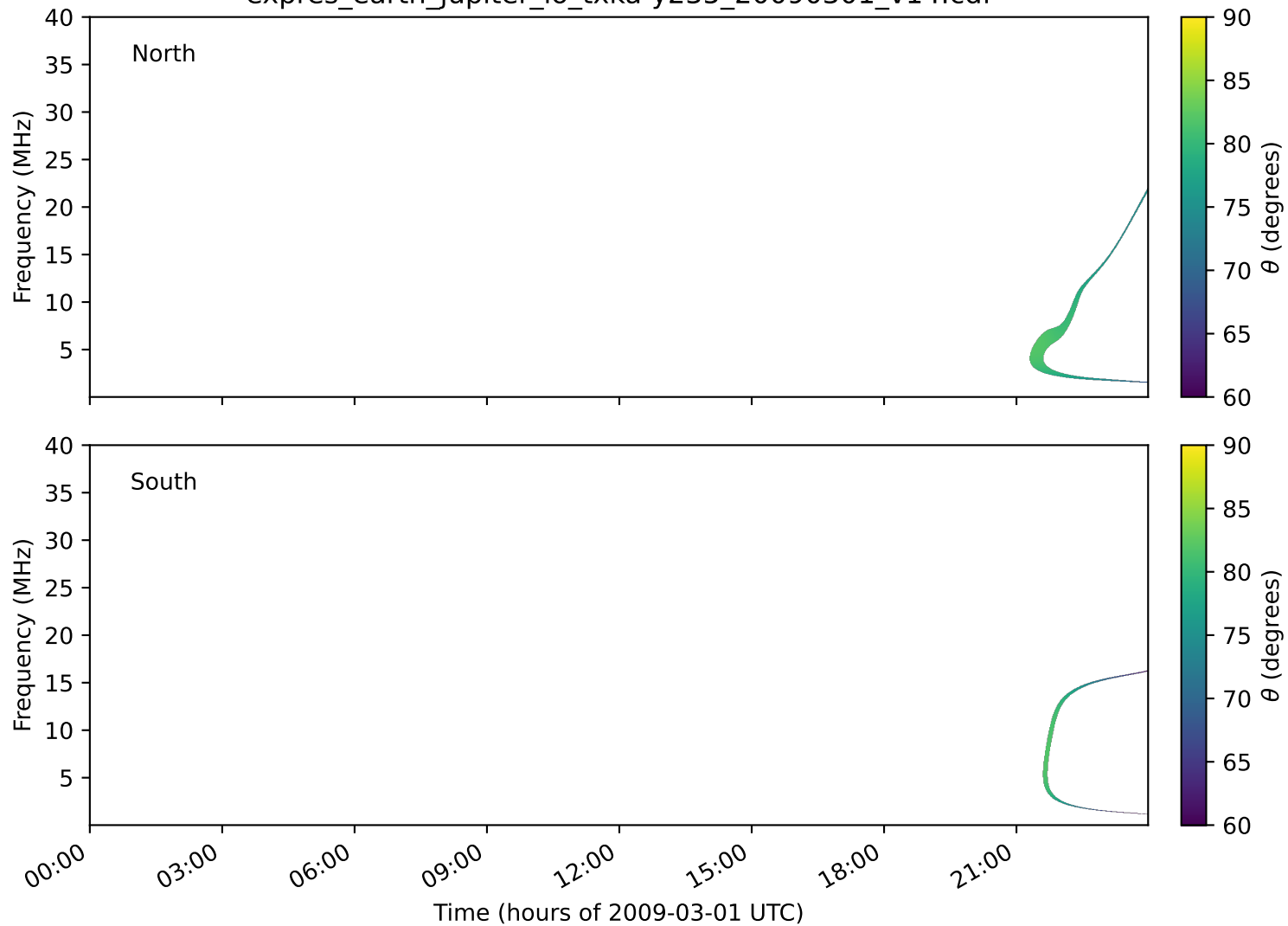
expres_earth_jupiter_io_txka-y235_20090301_v14.cdf
