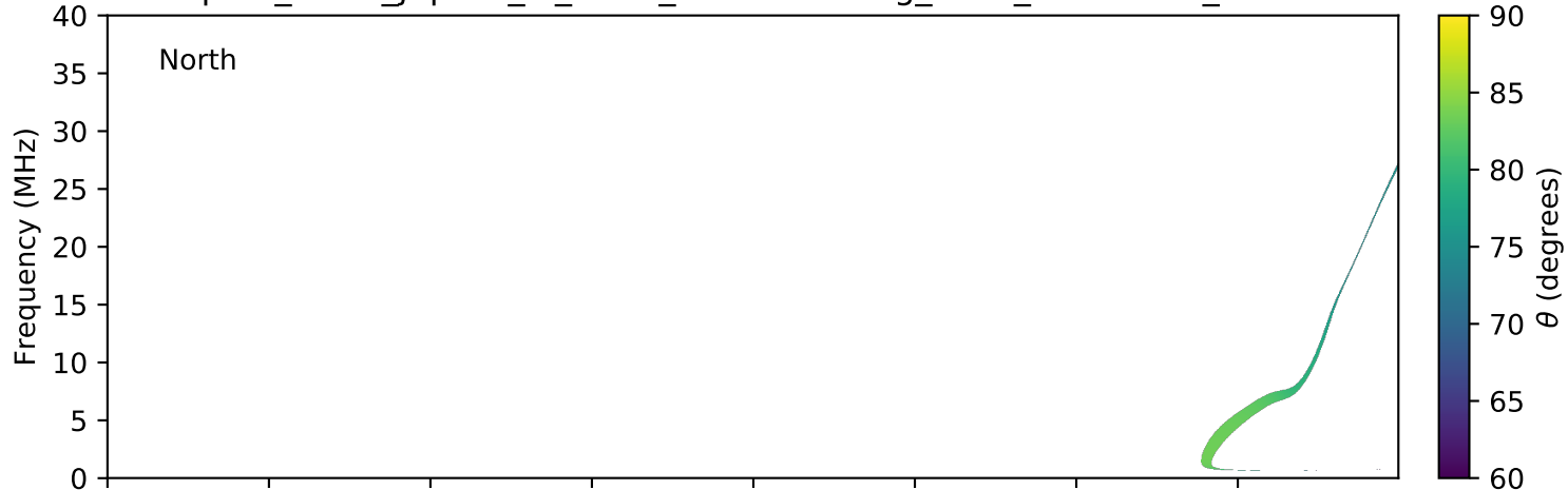
expres_earth_jupiter_io_isaac_lossc-wid1deg_3kev_20090324_v01.cdf
