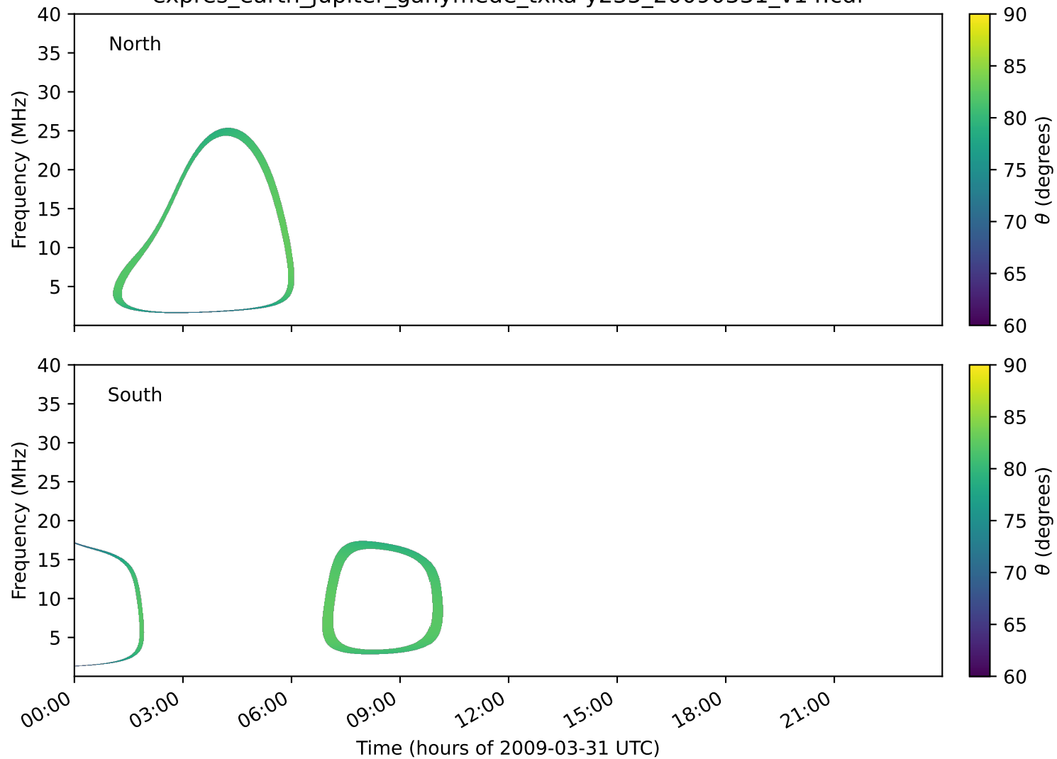
expres_earth_jupiter_ganymede_txka-y235_20090331_v14.cdf
