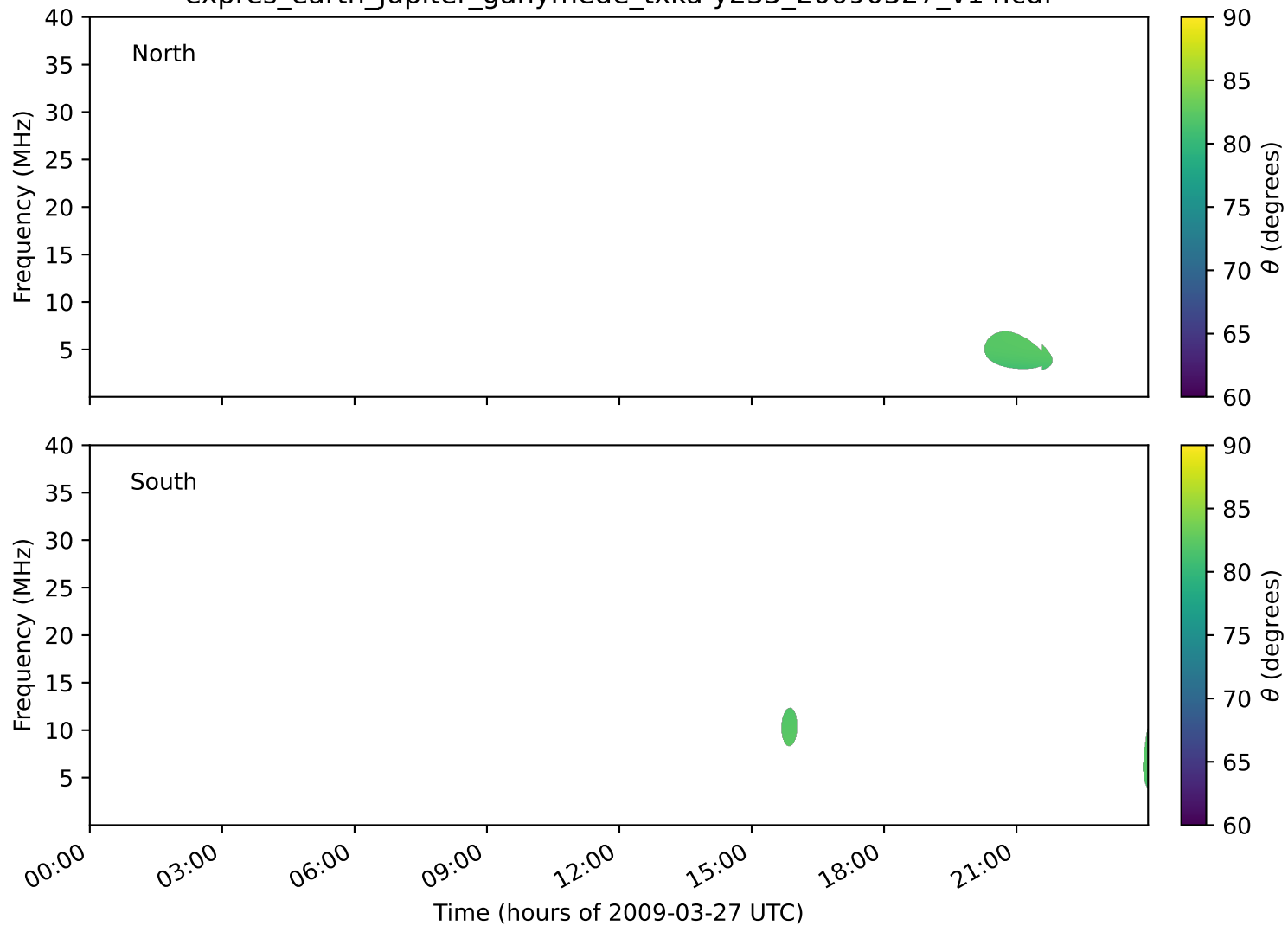
expres_earth_jupiter_ganymede_txka-y235_20090327_v14.cdf
