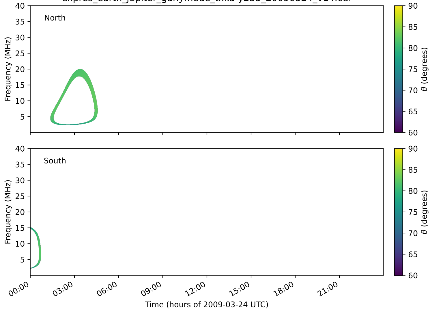
expres_earth_jupiter_ganymede_txka-y235_20090324_v14.cdf
