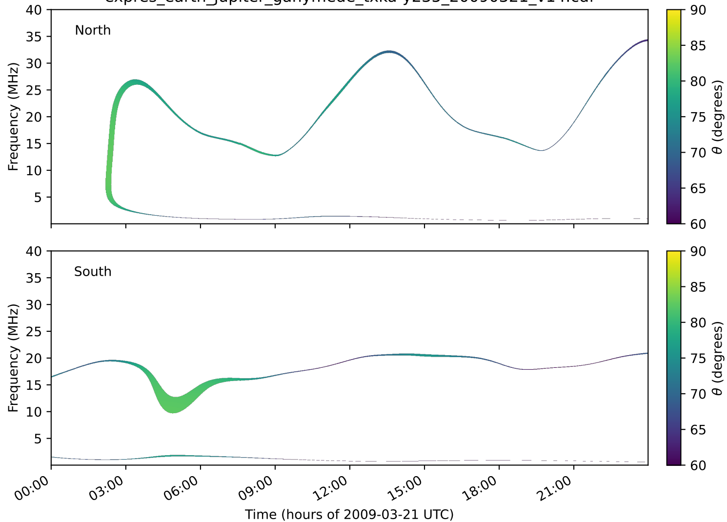
expres_earth_jupiter_ganymede_txka-y235_20090321_v14.cdf
