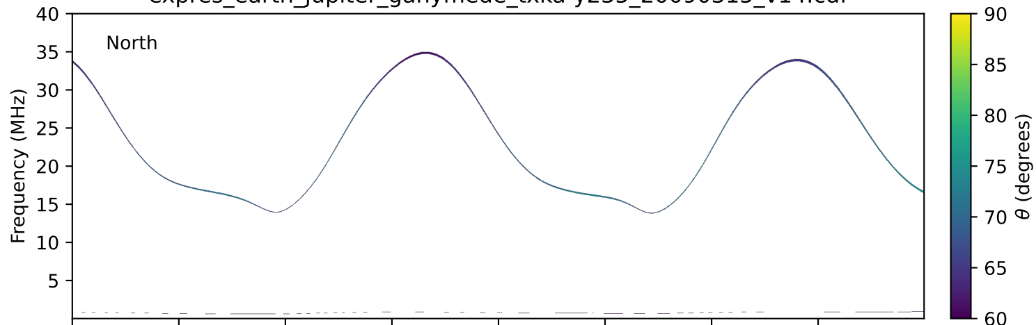
expres_earth_jupiter_ganymede_txka-y235_20090315_v14.cdf
