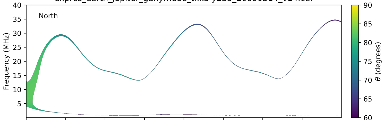
expres_earth_jupiter_ganymede_txka-y235_20090314_v14.cdf
