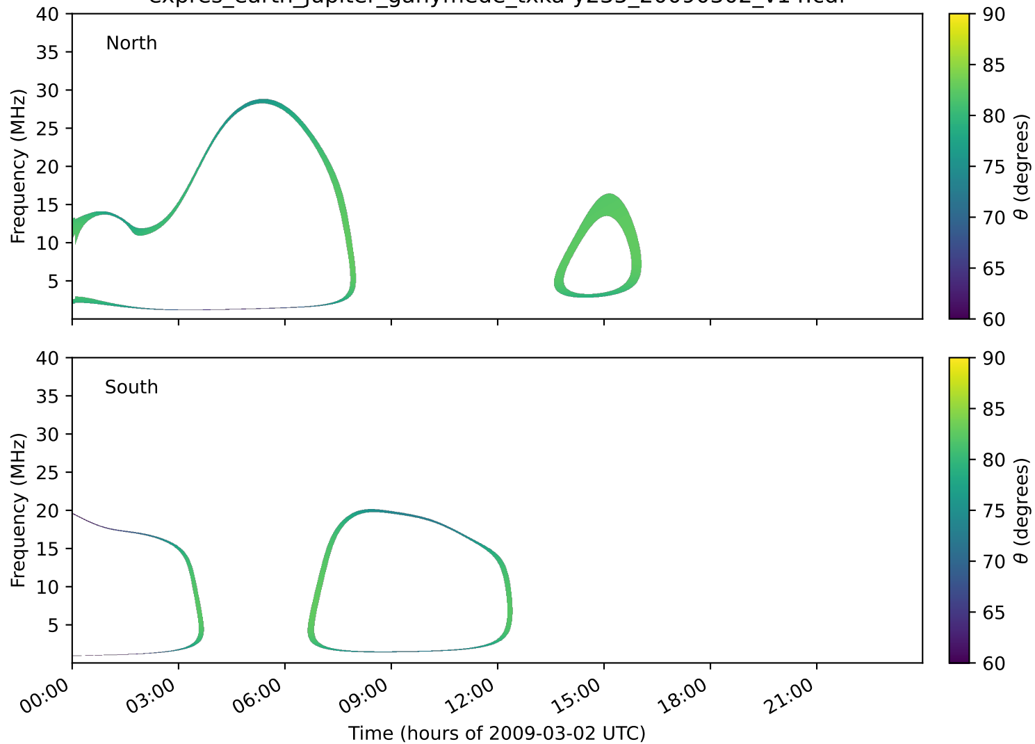
expres_earth_jupiter_ganymede_txka-y235_20090302_v14.cdf
