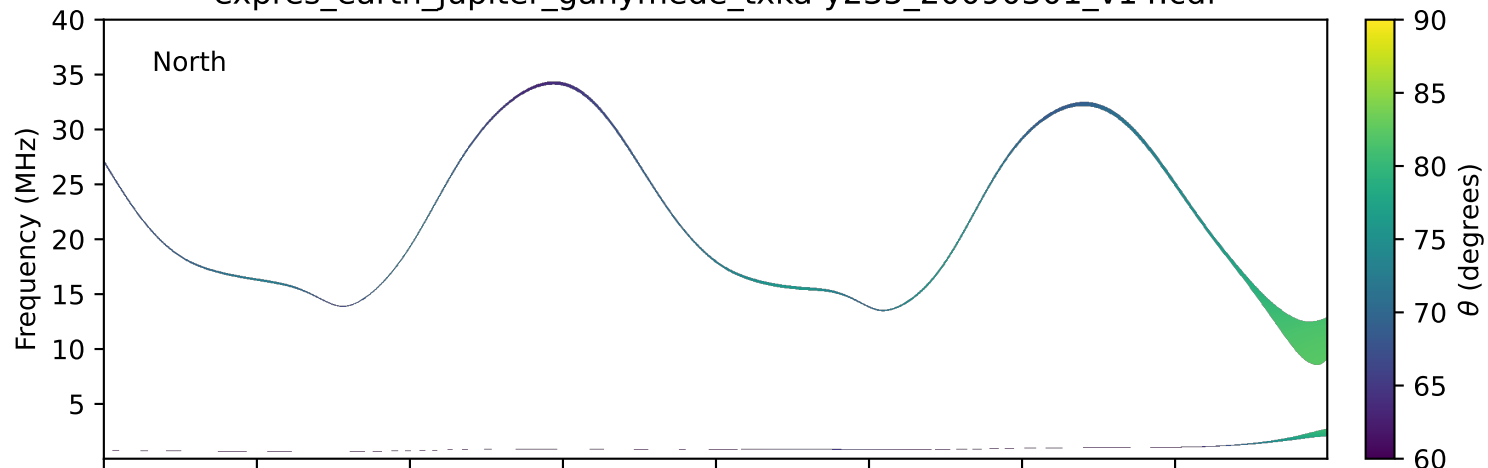
expres_earth_jupiter_ganymede_txka-y235_20090301_v14.cdf
