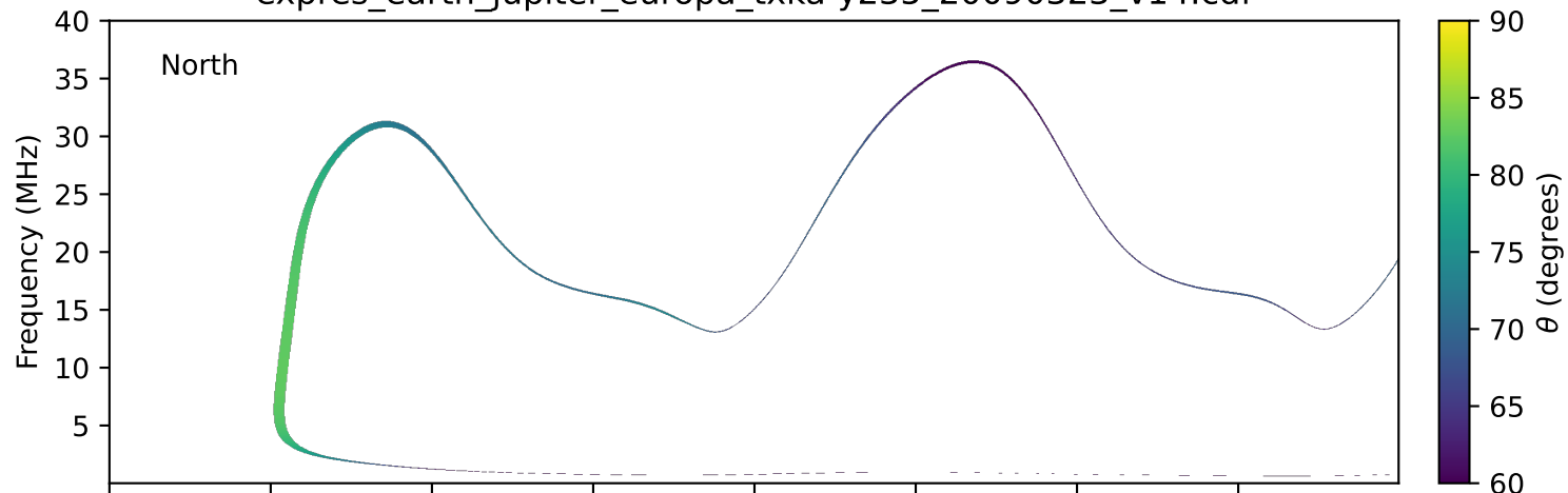
expres_earth_jupiter_europa_txka-y235_20090323_v14.cdf
