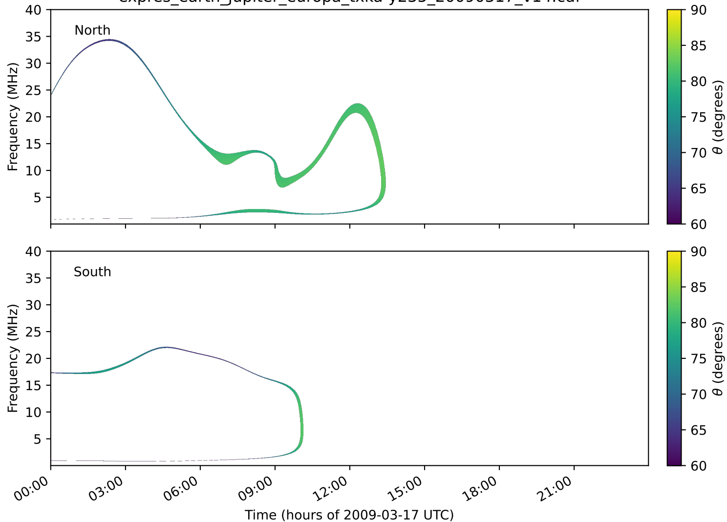
expres_earth_jupiter_europa_txka-y235_20090317_v14.cdf
