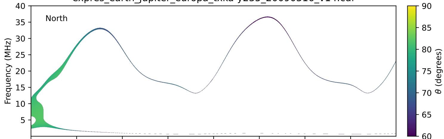
expres_earth_jupiter_europa_txka-y235_20090316_v14.cdf
