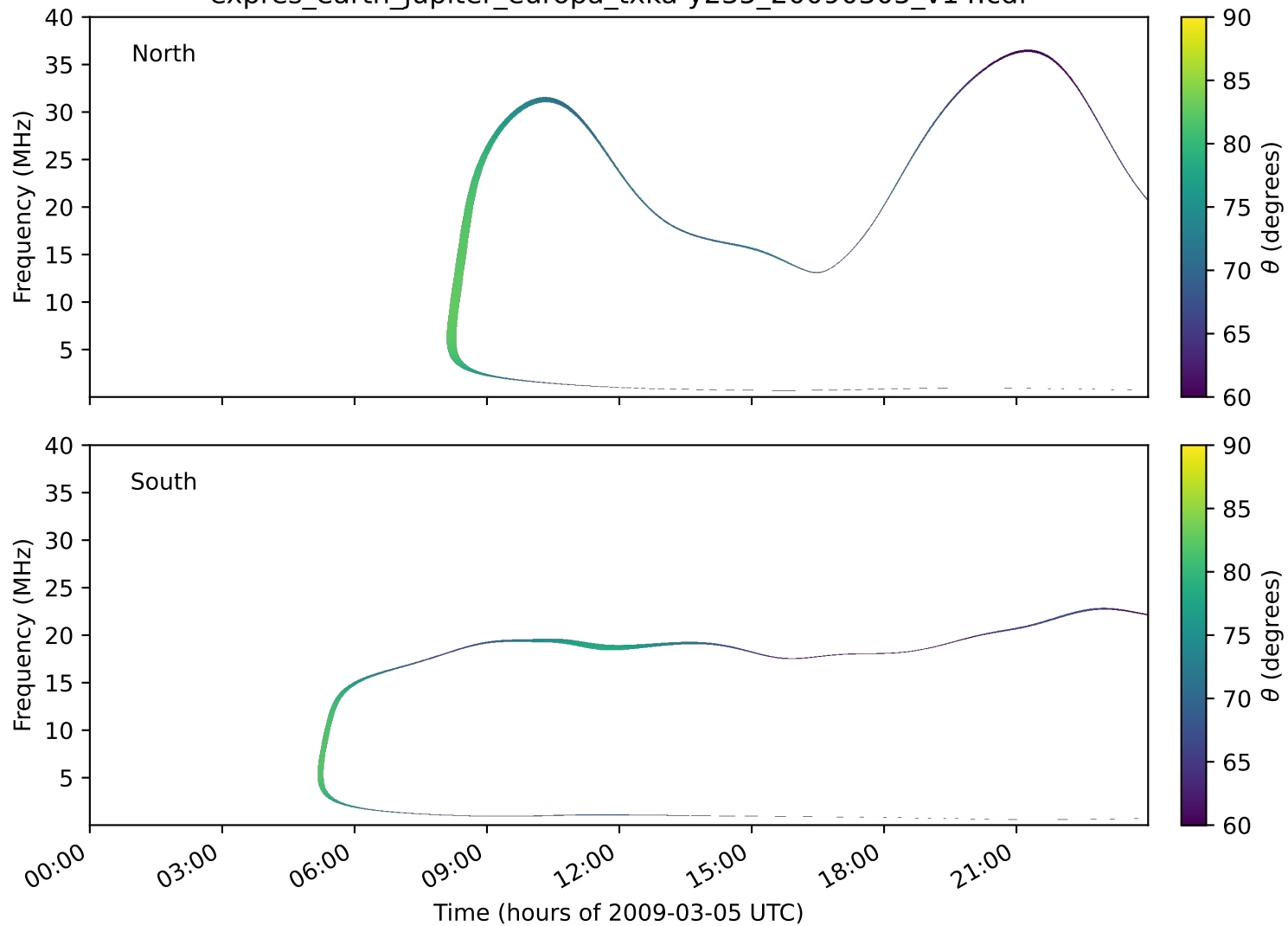
expres_earth_jupiter_europa_txka-y235_20090305_v14.cdf
