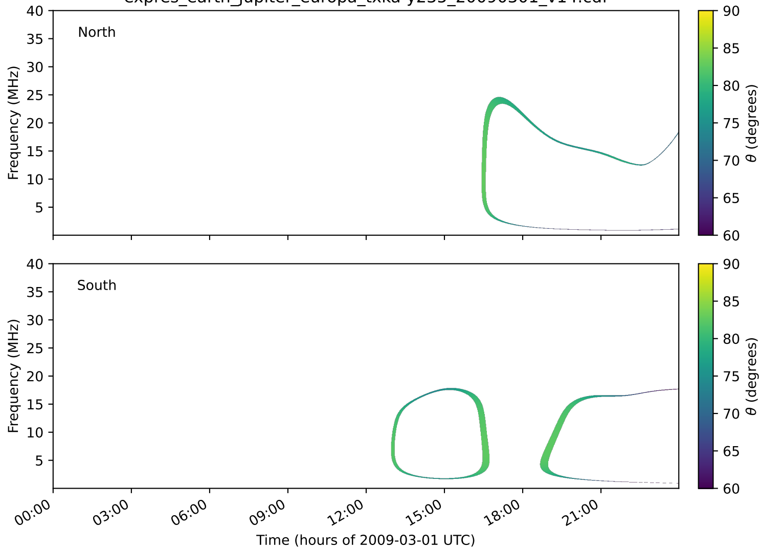
expres_earth_jupiter_europa_txka-y235_20090301_v14.cdf
