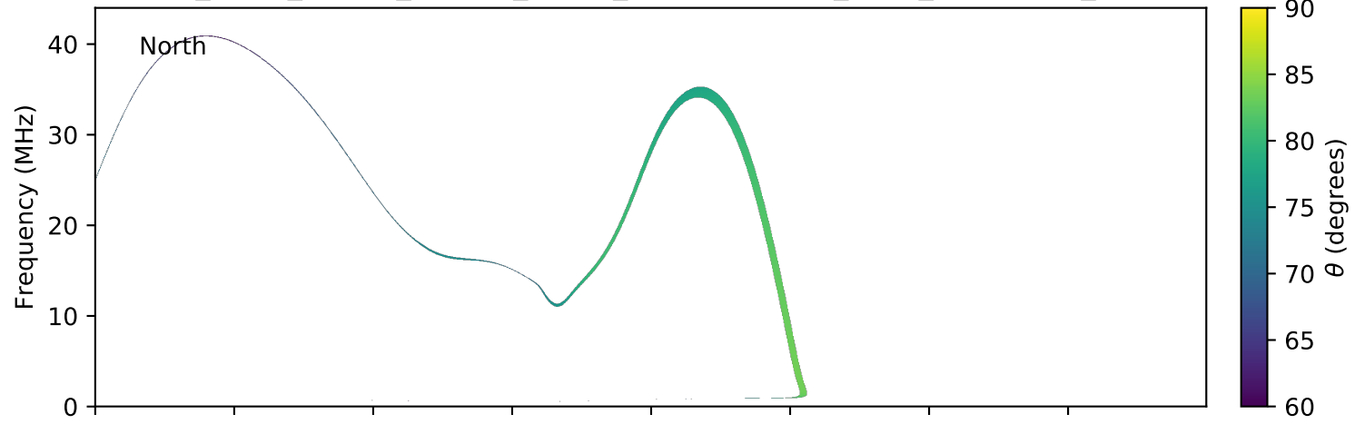
expres_earth_jupiter_europa_jrm09_lossc-wid1deg_3kev_20090324_v01.cdf
