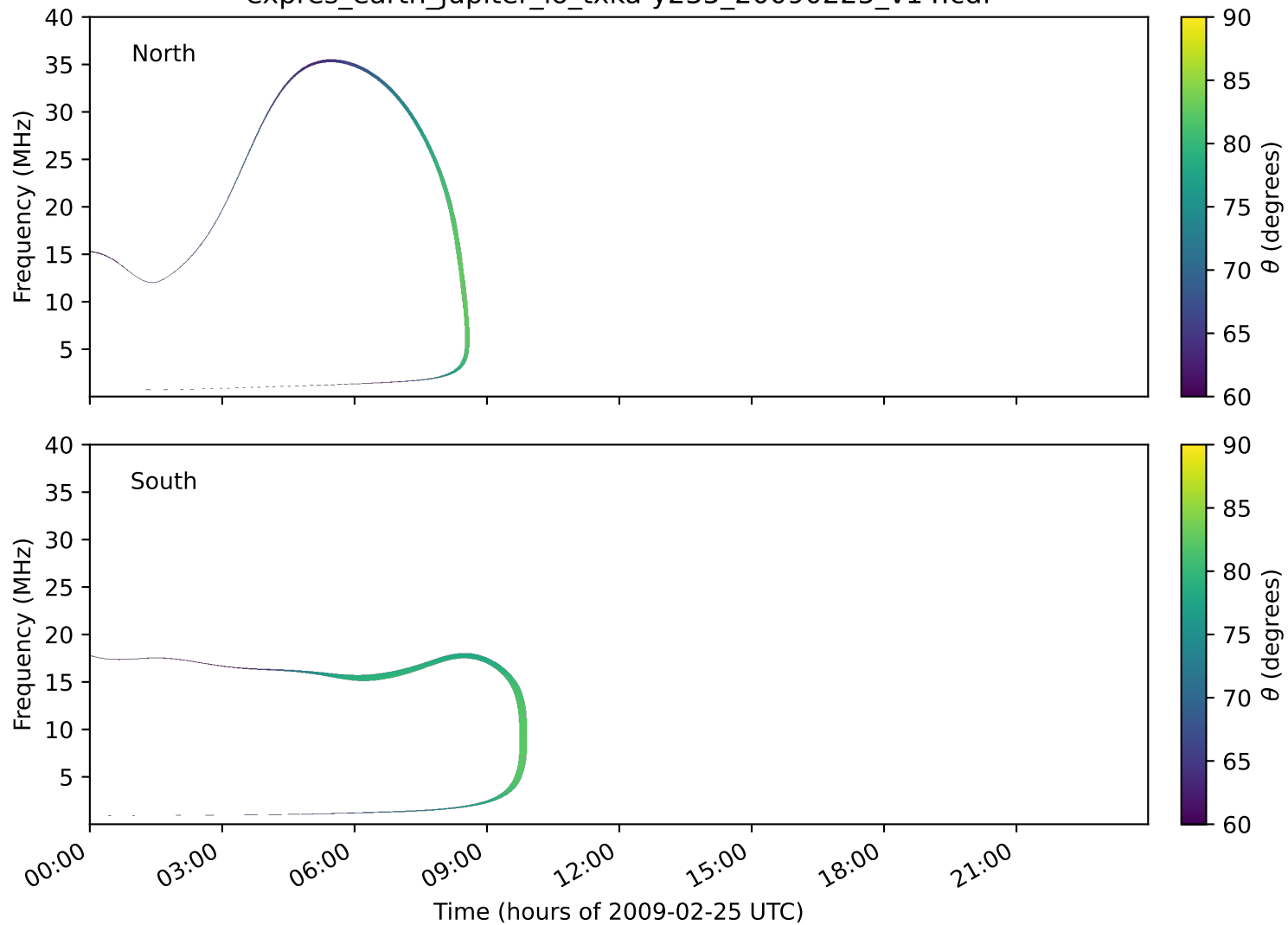
expres_earth_jupiter_io_txka-y235_20090225_v14.cdf
